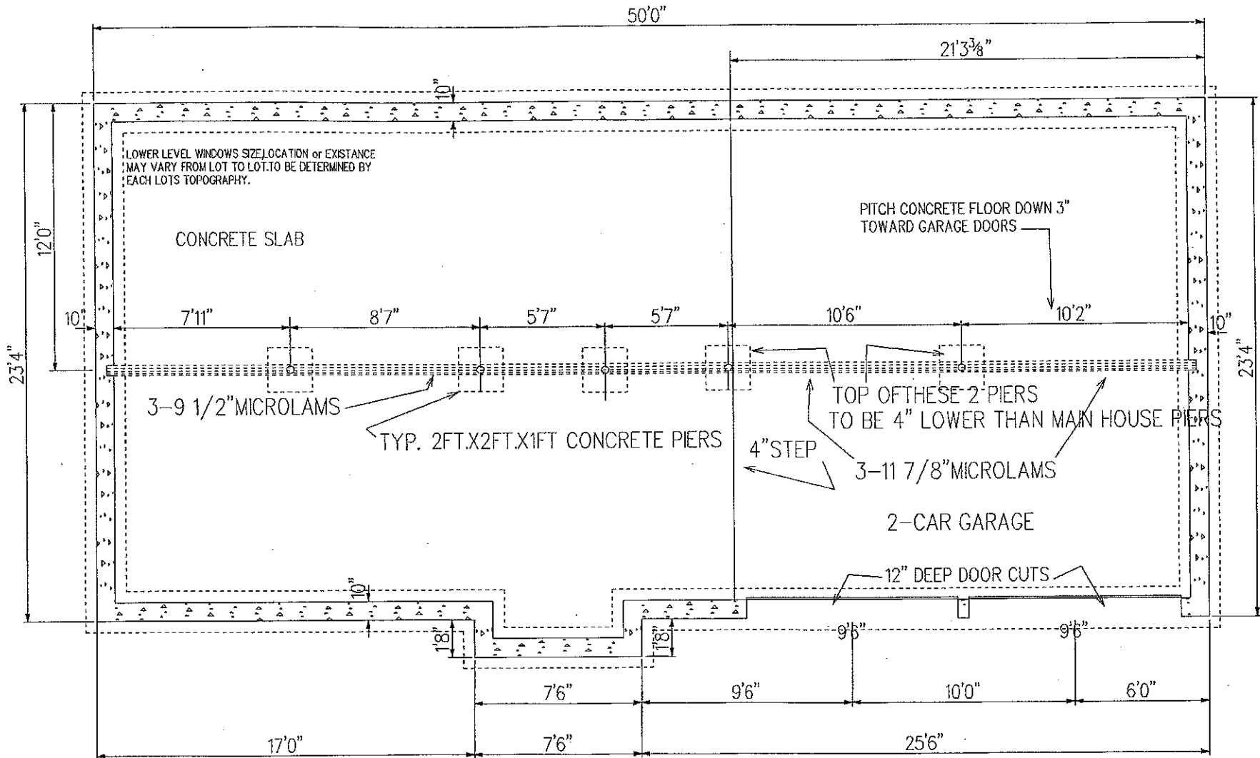
FOUNDATION PLAN MEADOW CREST
